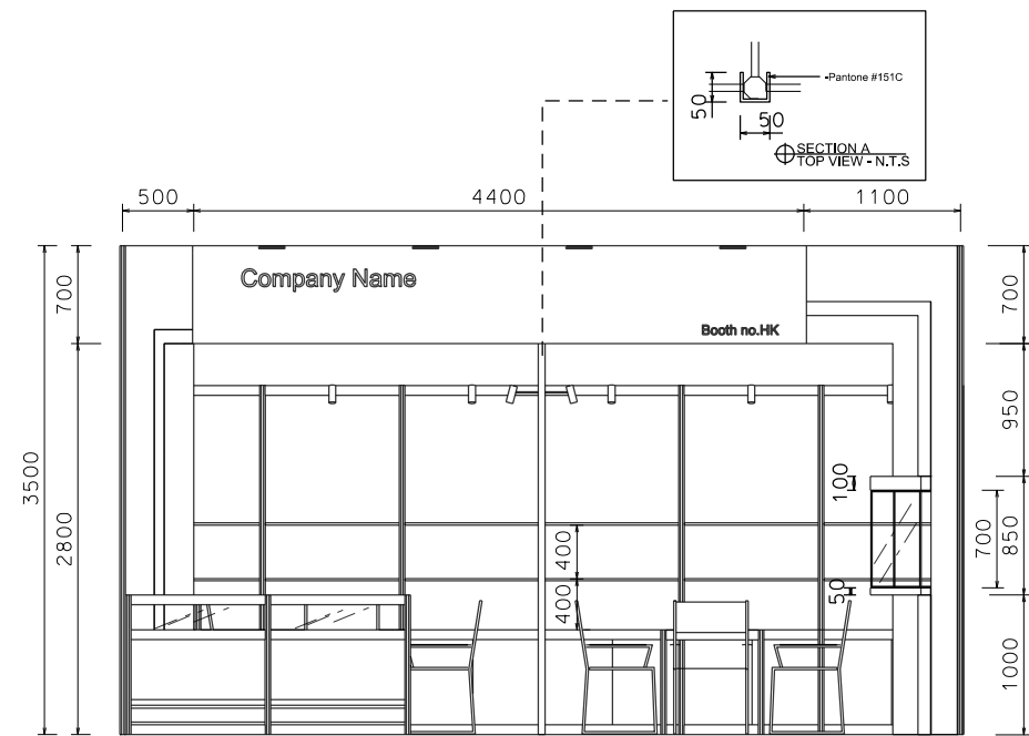
FRONT ELEVATION
